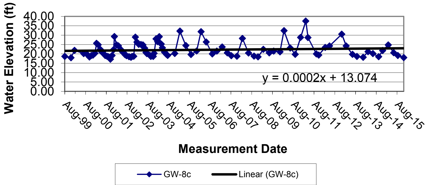
Figure 6h. Hydrograph for Well GW-8c
