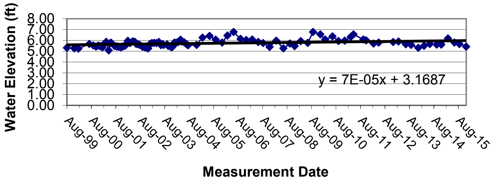
Figure 6j. Hydrograph for Well GW-10a
