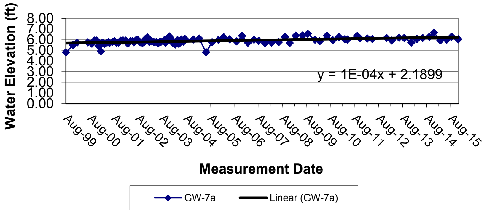
Figure 6g. Hydrograph for Well GW-7a
