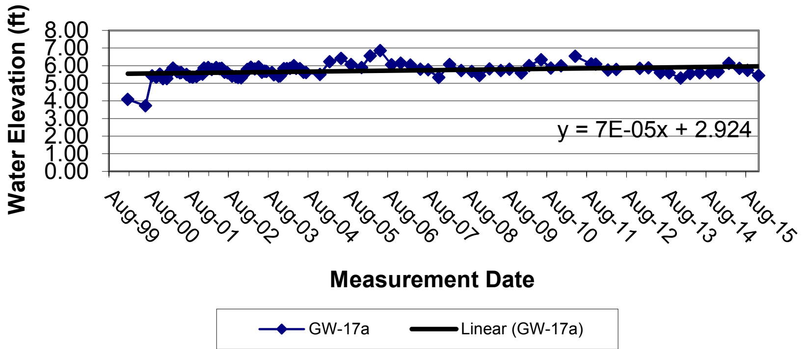
Figure 6q. Hydrograph for Well GW-17a
