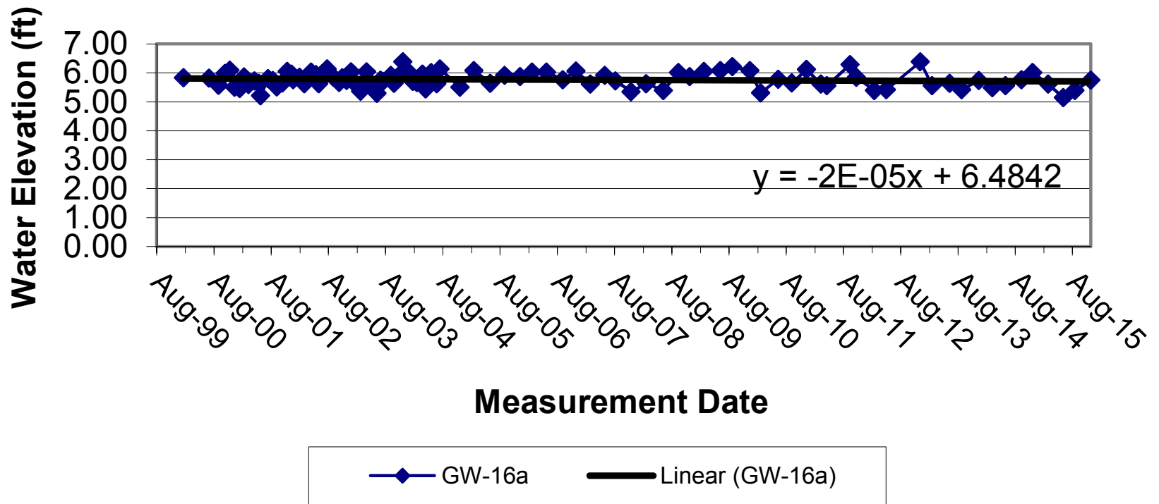
Figure 6p. Hydrograph for Well GW-16a
