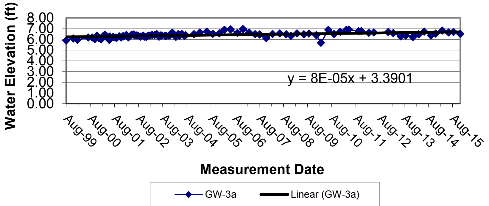
Figure 6c. Hydrograph for Well GW-3a
