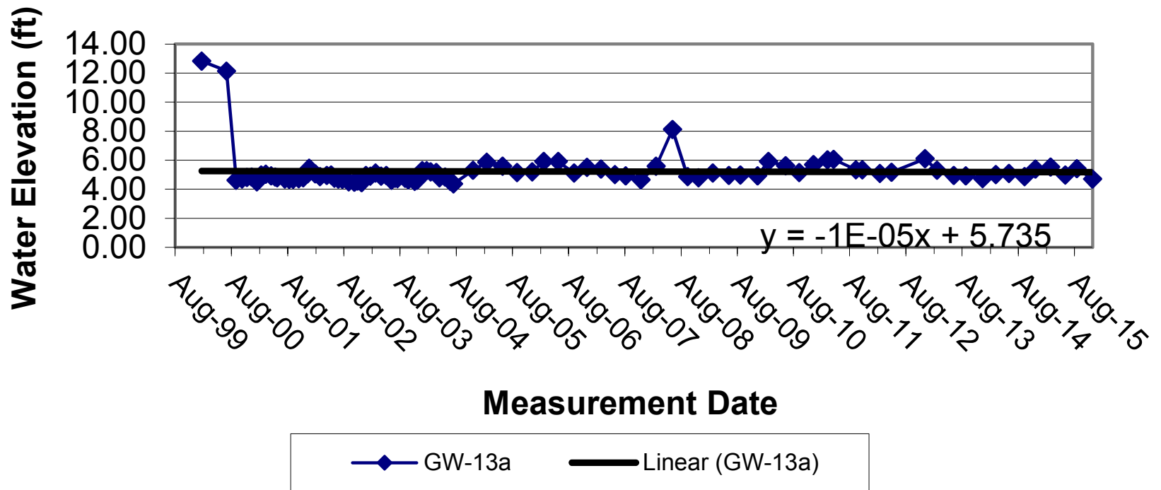
Figure 6m. Hydrograph for Well GW-13a
