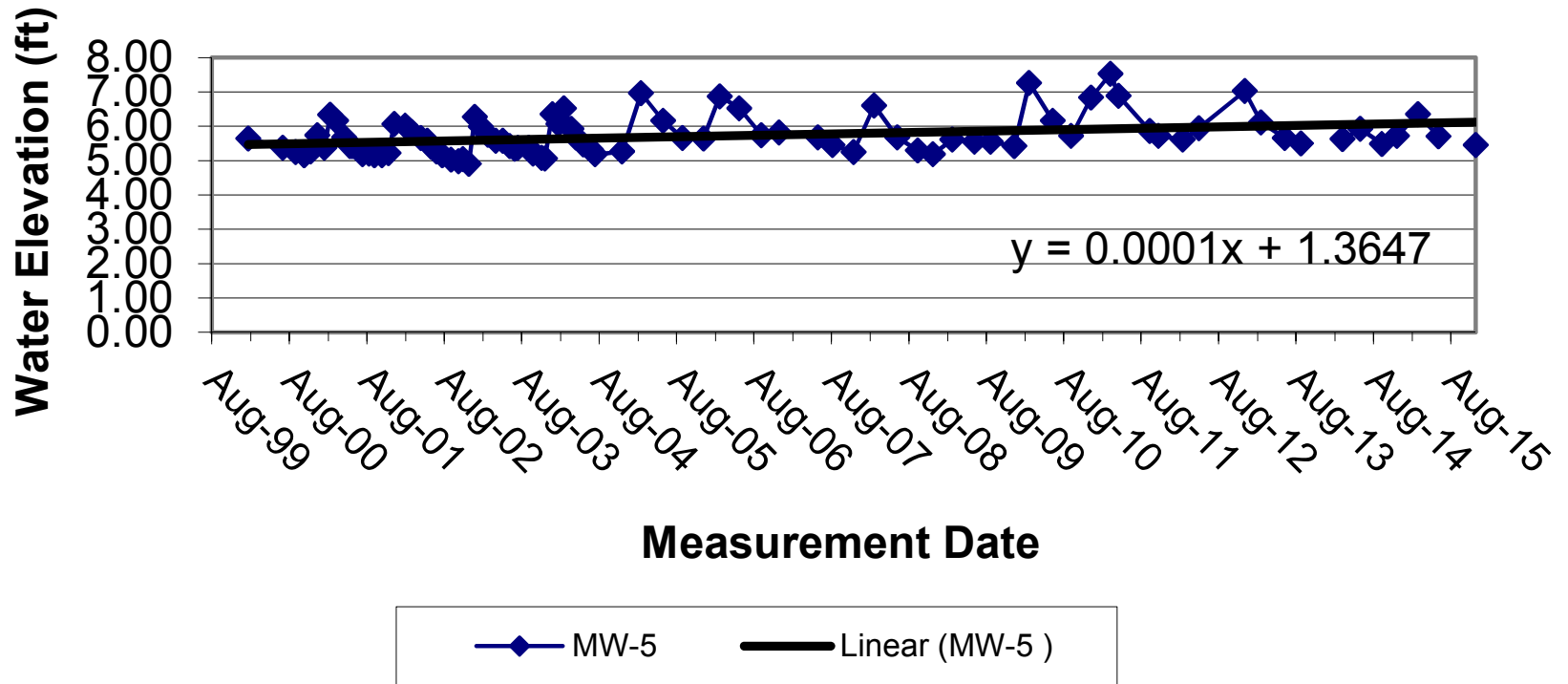
Figure 6r. Hydrograph for Well MW-5
