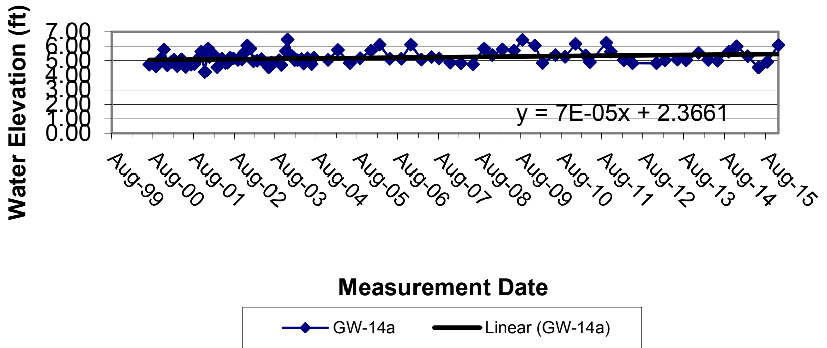
Figure 6n. Hydrograph for Well GW-14a
