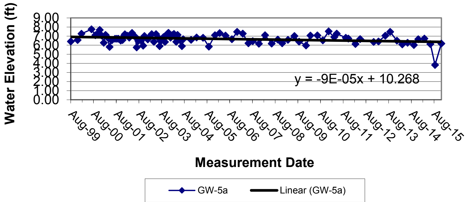
Figure 6e. Hydrograph for Well GW-5a
